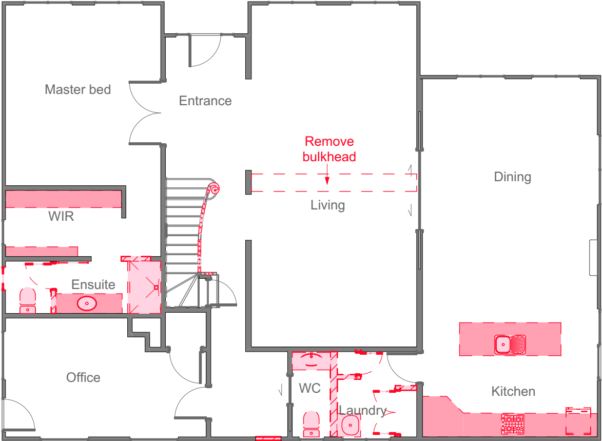
1 Existing & Demo Plan 1:100
