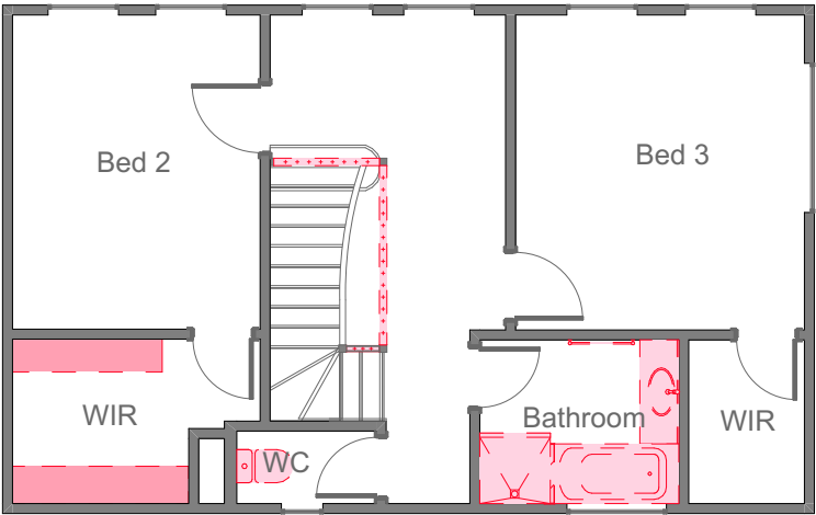
1 Existing & Demo 1st Floor 1:100
